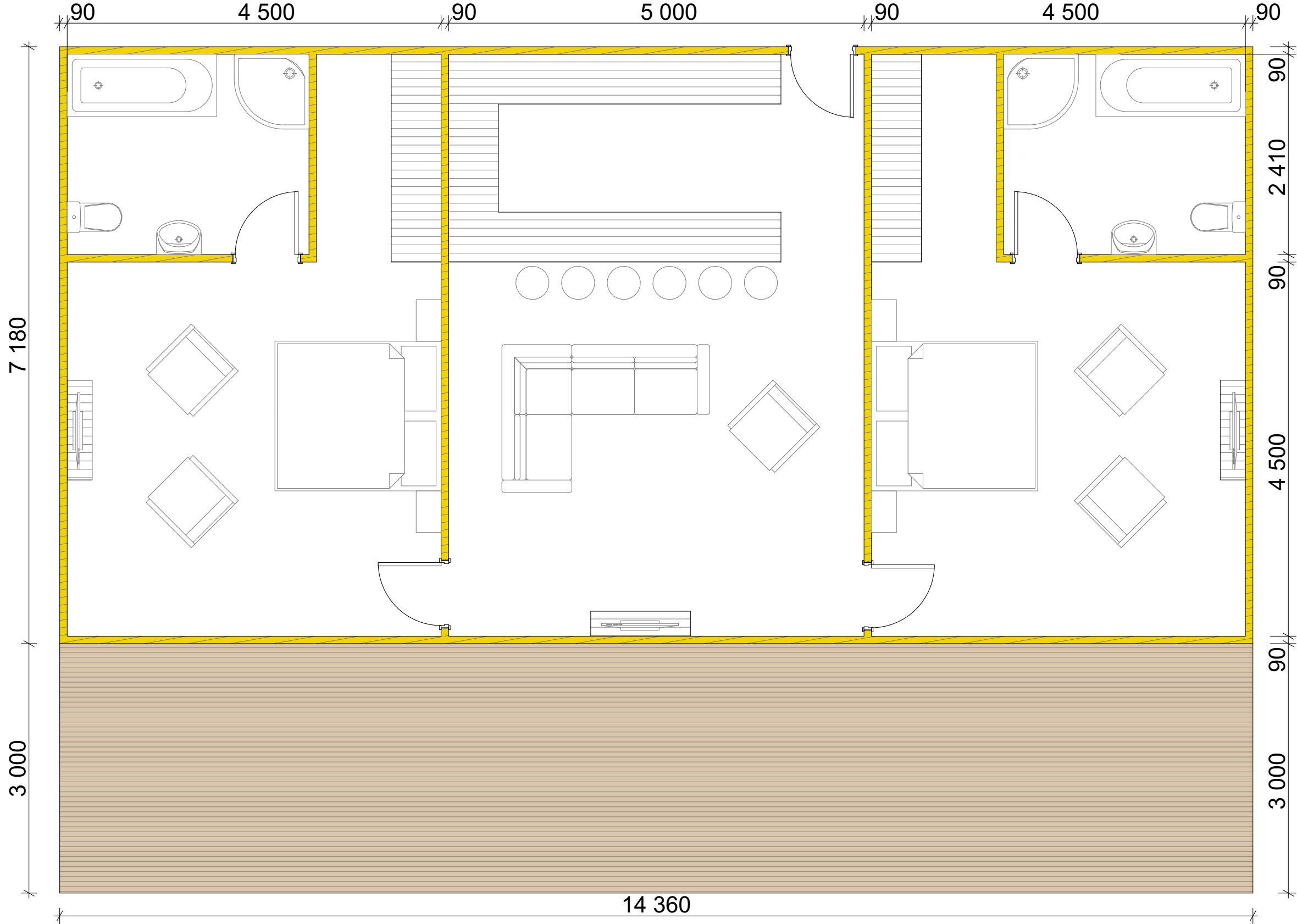
GROUND FLOOR PLAN AREA 103.1m 2
